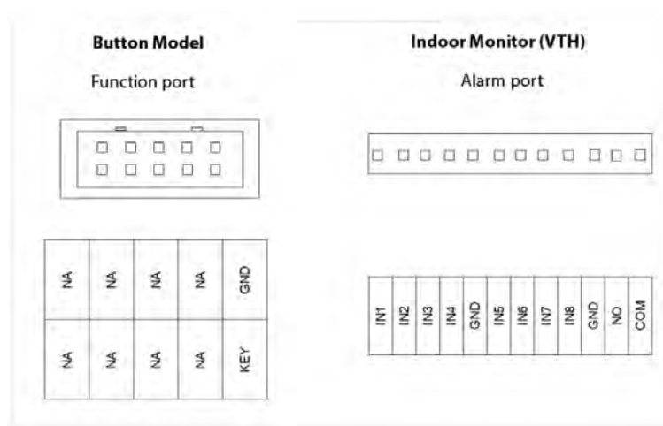
Figure 13-2 Cable connection
